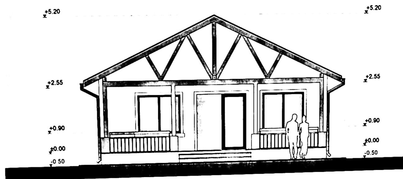
FATADA PRINCIPALA
